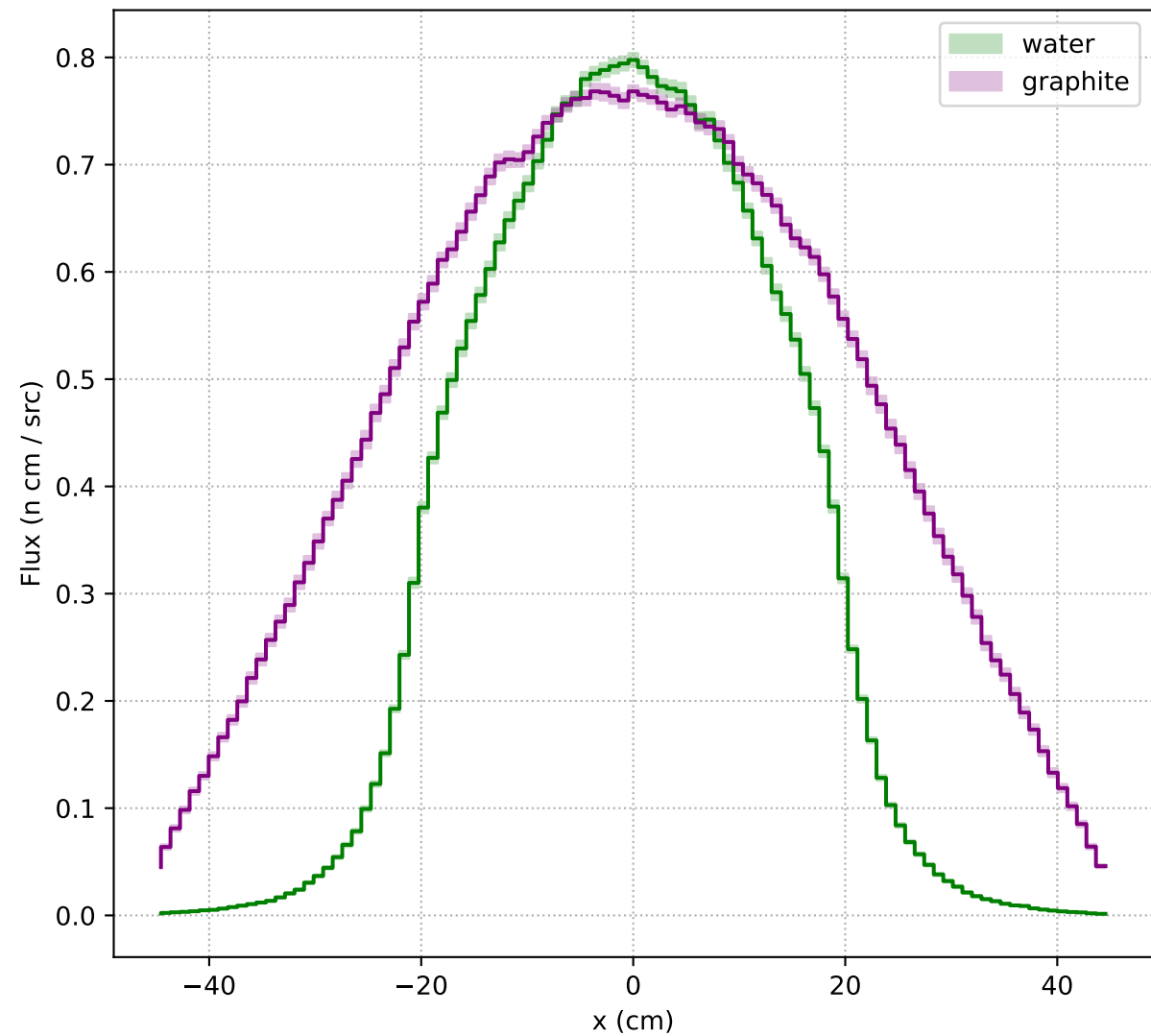
Fast neutrons
